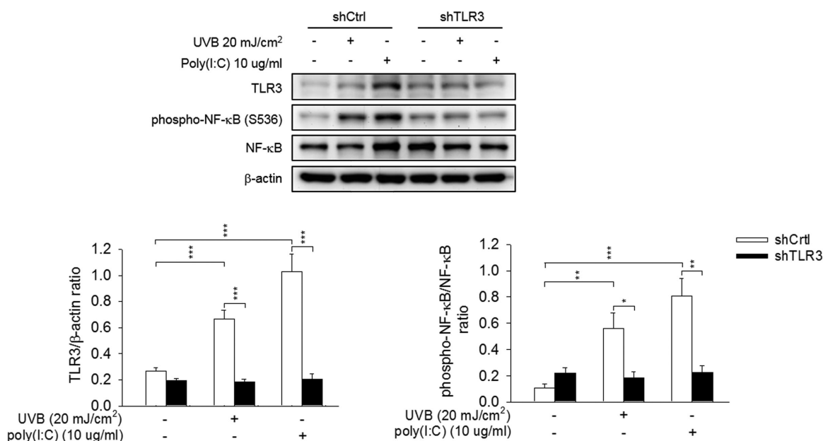
FIGURE 4. Western blotting analysis of TLR3 and phospho-NF- \kappa B in cultured PECs with TLR3 knockdown using shTLR3 transfection and in PECs without TLR3 knockdown using non-targeting shRNA (shCtrl, control group) transfection. The expression of TLR3 and phospho-NF- \kappa B was analyzed in these cells (shTLR3 and shCtrl) 24 hours after UVB irradiation (20 mJ/cm 2 ) or 24 hours after treatment with poly(I:C) (10 \mu g/mL) ( n = 6 ; * P < 0.05 , ** P < 0.01 , *** P < 0.001 ). Comparisons were made using Student's t -test. Data are presented as means \pm SEM. All experiments were repeated with similar results.
